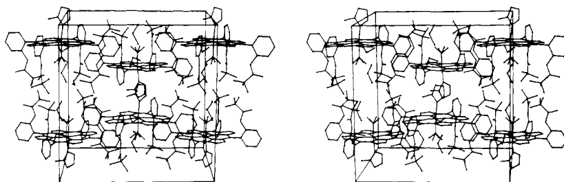
Figure 7. Stereodiagram of the unit cell for \text{Fe}(\text{O}_2)(\text{TpivPP})(2\text{-MeIm})\text{-EtOH} . The two crystallographically independent ethanol moieties are shown; disorder of the terminal oxygen atom but not of the 2-MeIm is shown. Hydrogen atoms are omitted for clarity. The view is approximately down the c axis; the b axis is vertical.
