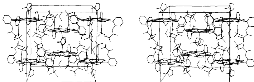
Figure 6. Stereodiagram of the unit cell for \text{Fe}(\text{TpivPP})(2\text{-MeIm})\text{-EtOH} . The two crystallographically independent ethanol moieties are shown. Hydrogen atoms are omitted for clarity. The view is approximately down the c axis; the b axis is vertical.
