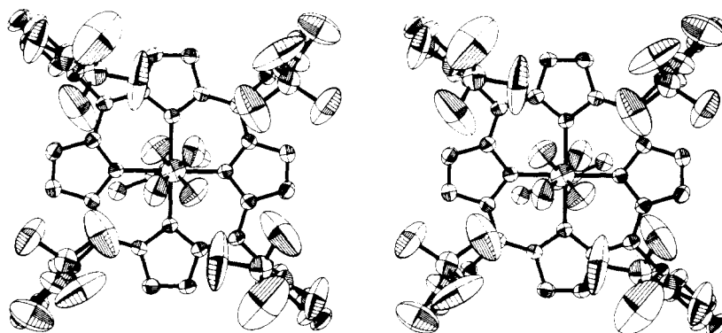
Figure 5. Stereodiagram of \text{Fe}(\text{O}_2)(\text{TpivPP})(2\text{-MeIm}) looking down the twofold axis. Ellipsoids are drawn at the 30% probability level. Disorder of the terminal oxygen atom but not of the 2-MeIm is shown. Hydrogen atoms are omitted for clarity.
