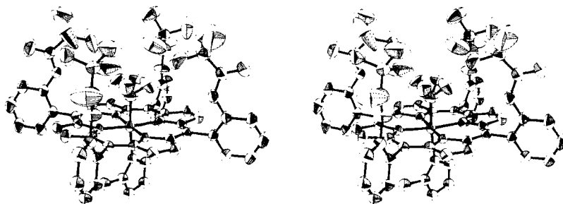
Figure 4. Stereodiagram of \text{Fe}(\text{O}_2)(\text{TpivPP})(2\text{-MeIm}) . Ellipsoids are drawn at the 30% probability level. Disorder of the terminal oxygen atom but not of the 2-MeIm is shown. Hydrogen atoms are omitted for clarity.
