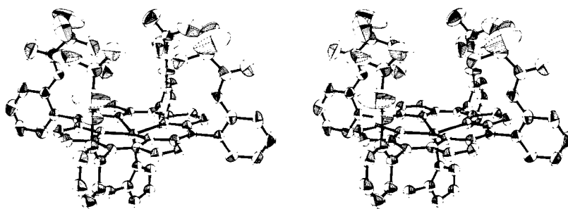
Figure 2. Stereodiagram of Fe(TpivPP)(2-MeIm) . Ellipsoids are drawn at the 30% probability level. Hydrogen atoms are omitted for clarity.
