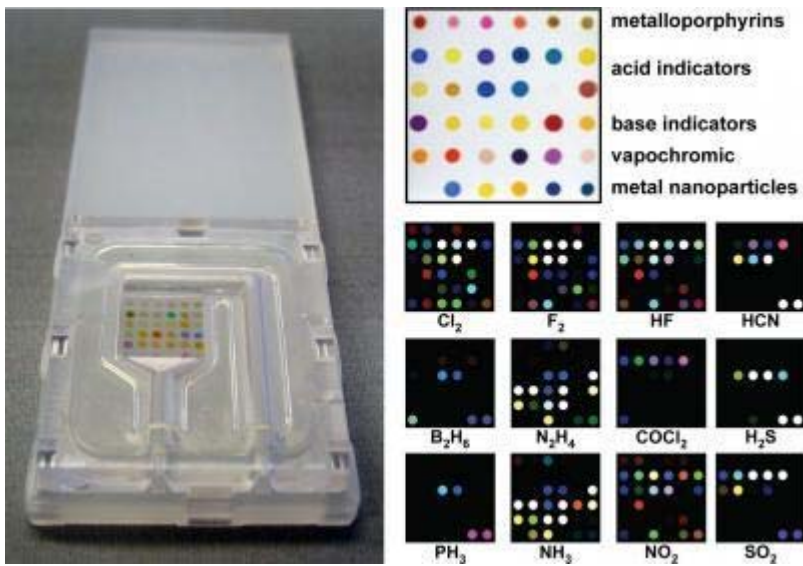
The device uses a printed array smaller than a postage stamp made up of nanoporous pigments that change color in response to their chemical environment. The color differences are shown for a few representative poison gases
